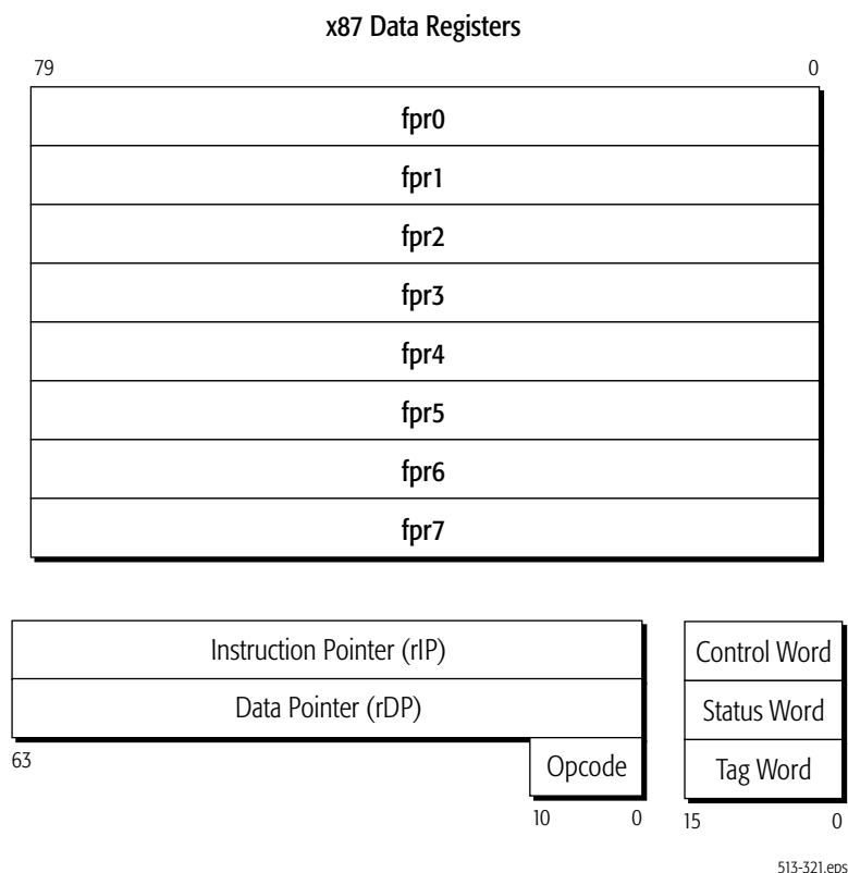
Figure 6-1. x87 Registers
